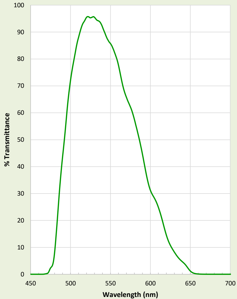
Astrodon Johnson-Cousins V Filter
