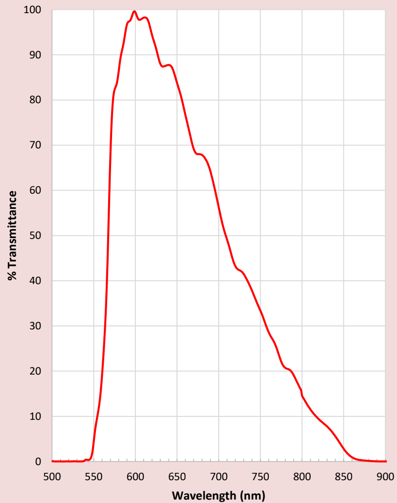
Astrodon Johnson-Cousins Rc Filter
