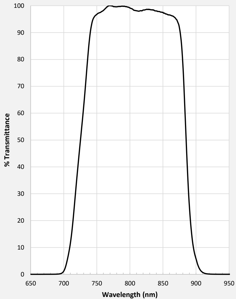
Astrodon Johnson-Cousins Ic Filter
