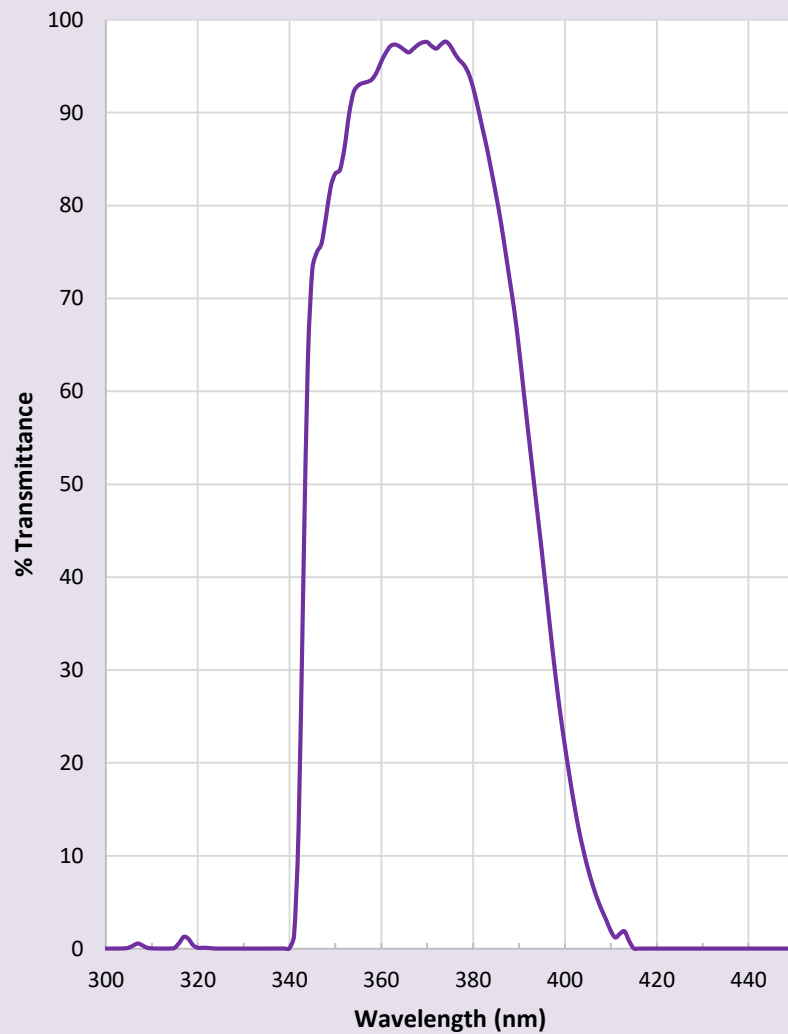
Astrodon Johnson-Cousins UV Filter
