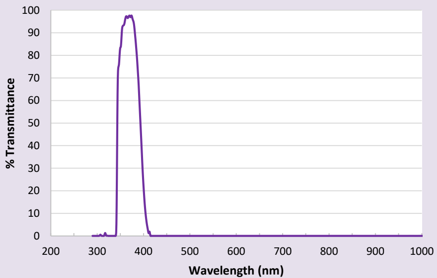
Astrodon Johnson-Cousins UV Filter
