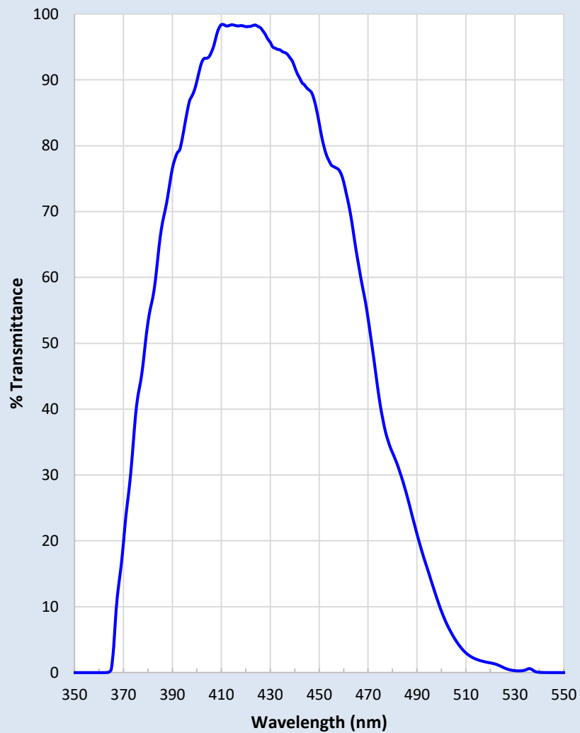
Astrodon Johnson-Cousins B Filter
