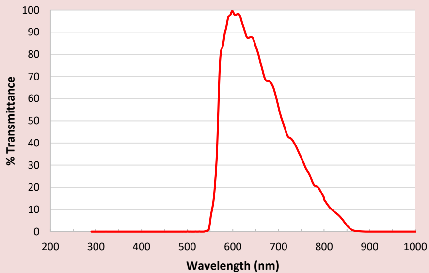
Astrodon Johnson-Cousins Rc Filter
