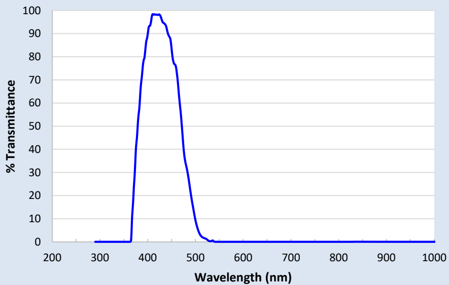
Astrodon Johnson-Cousins B Filter
