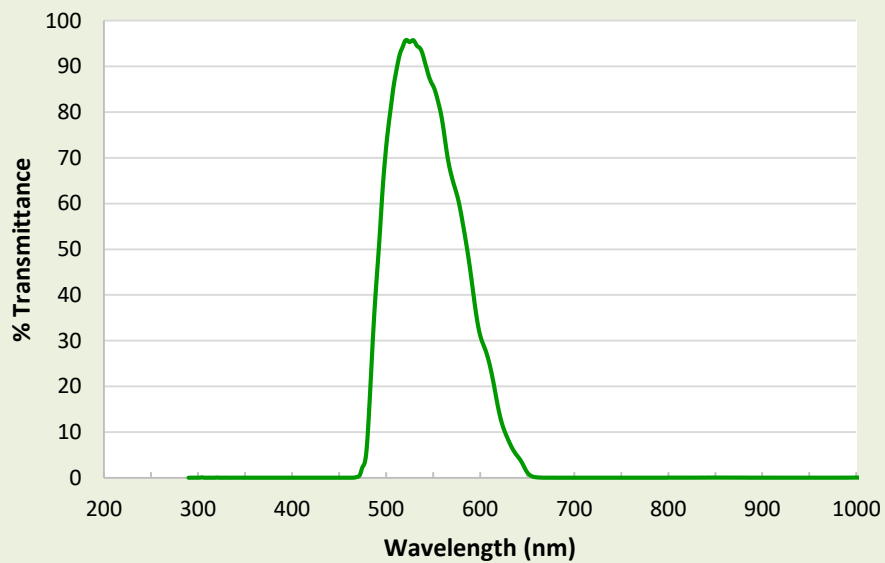
Astrodon Johnson-Cousins V Filter
