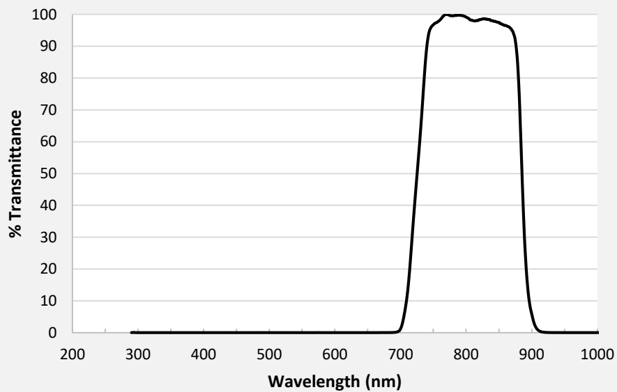
Astrodon Johnson-Cousins Ic Filter
